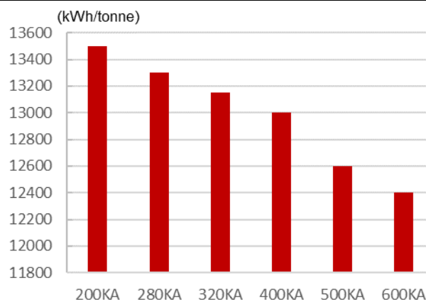
Figure 31: Power consumption for different types of electrolyzer
