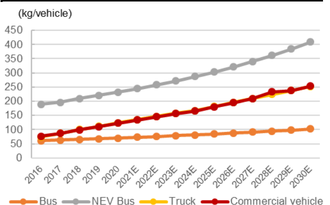
Figure 43: Aluminum consumption per commercial vehicle
